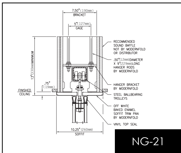
#14 Track System Bracket Mount (Smart Track Shown)
