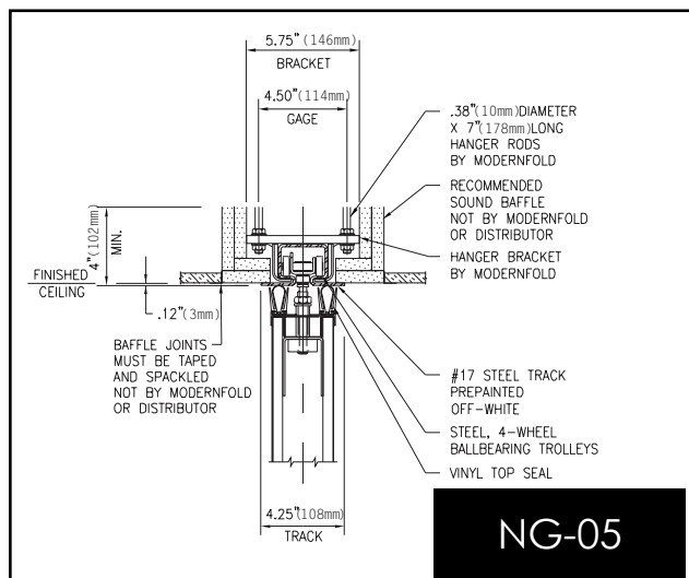
#17 Track System Bracket Mount (Smart Track Shown)
