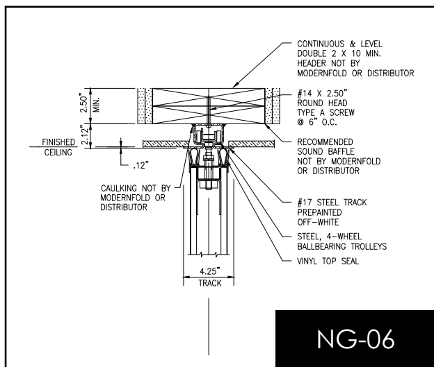
#17 Track System Direct Mount (Right Angle Shown)
